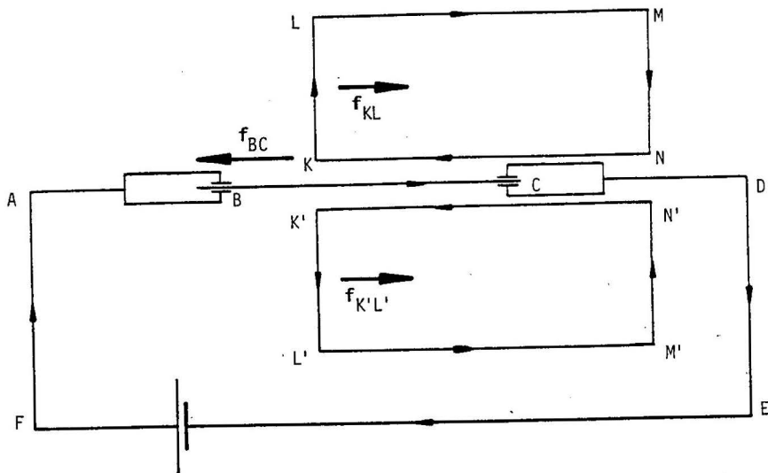
Fig. 79. Fourth Nicolaev's experiment.
