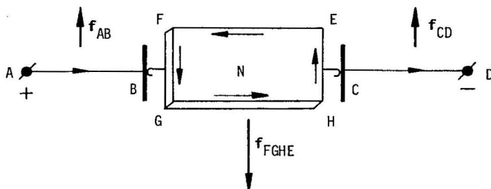
Fig. 71. Sigalov's third experiment.
