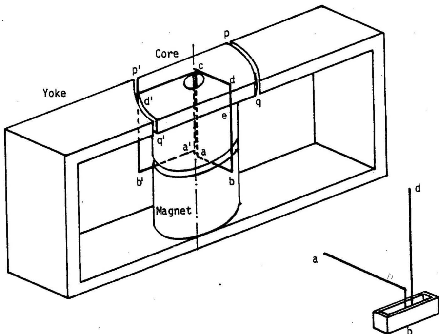
Fig. 29. Miller's one-and-a-half polar machine.
