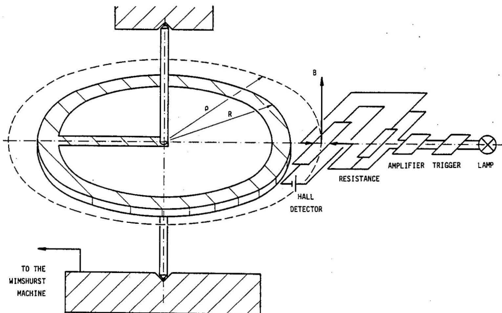
Fig. 23. Diagram of the apparatus for experiments.
