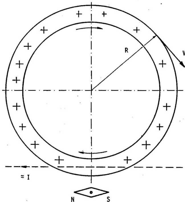
Fig. 21. The direct Rowland experiment.
