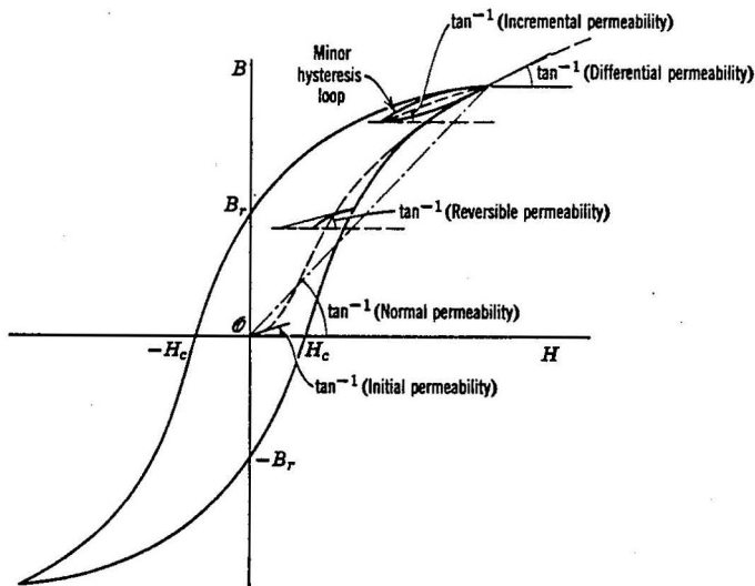
Fig. 3. The hysteresis loop.
