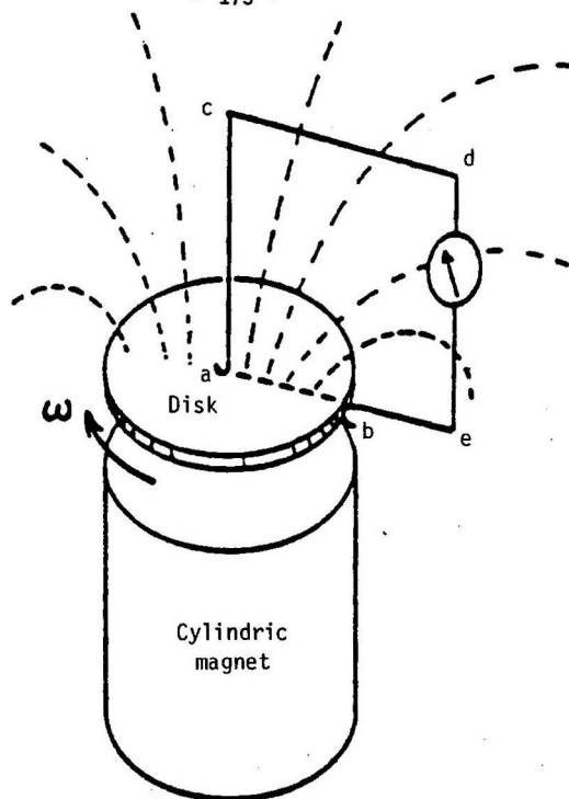
Fig. 24. Open half polar machine.
