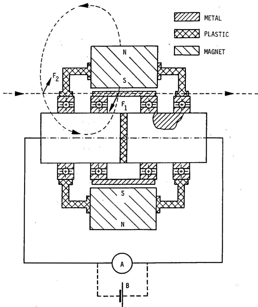
Fig. 37. Diagram of the demonstrational unipolar Marinov-Müller machine.
