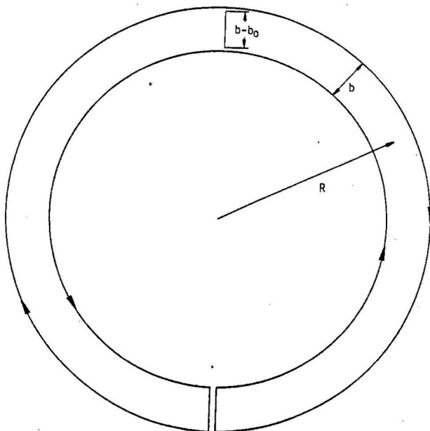
Fig. 4. Kennard's experiment.
