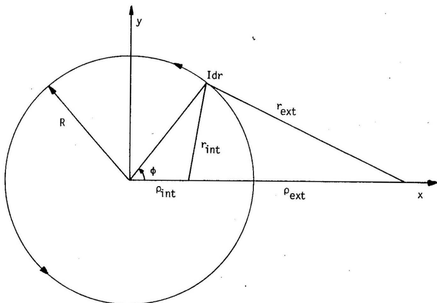
Fig. 2. Circular loop in which current flows.
