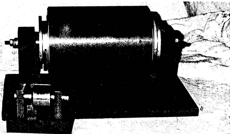
Fig. 96. Photograph of small and big ball-bearing motors.
