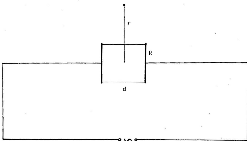
Fig. 89. Diagram of the experiment showing that polarization current does not act with potential magnetic forces on other currents.
