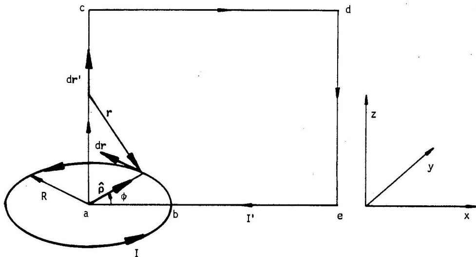
Fig. 9. Rectangular and circular circuits.
