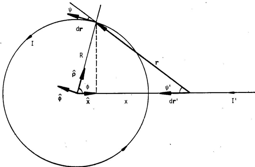
Fig. 13. Action of external radial current on circular current.
