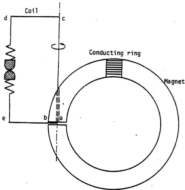
Fig. 25. Closed half polar machine.
