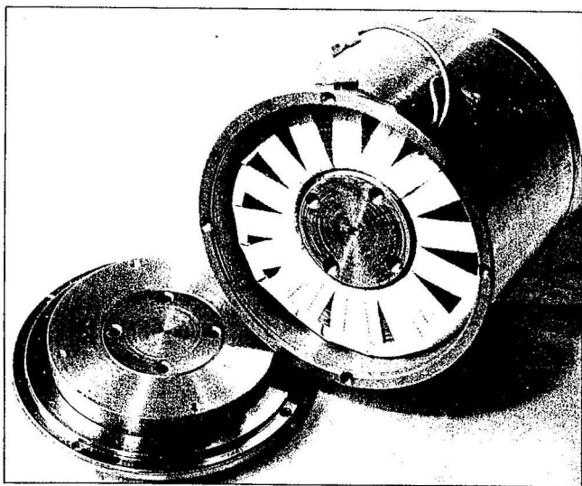
Fig. 93. Photograph of the BUL-CUB machine without stator with dismounted lower lid.
