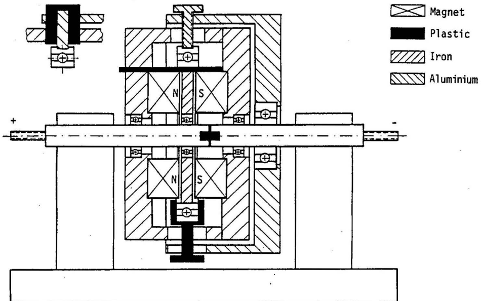
Fig. 33. Diagram of the demonstrational closed half polar Faraday-Bairlow machine.
